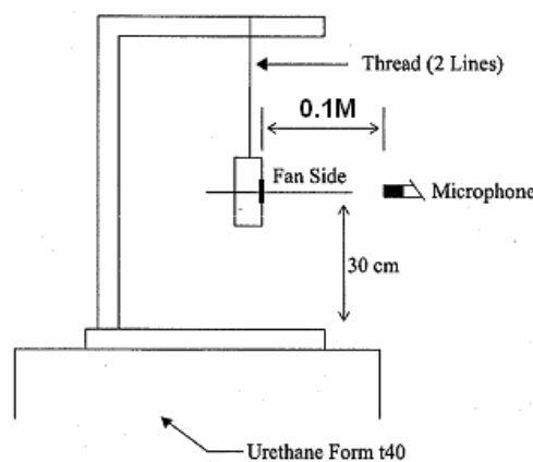
0.1 METER FROM MICROPHONE TO FAN INTAKE
