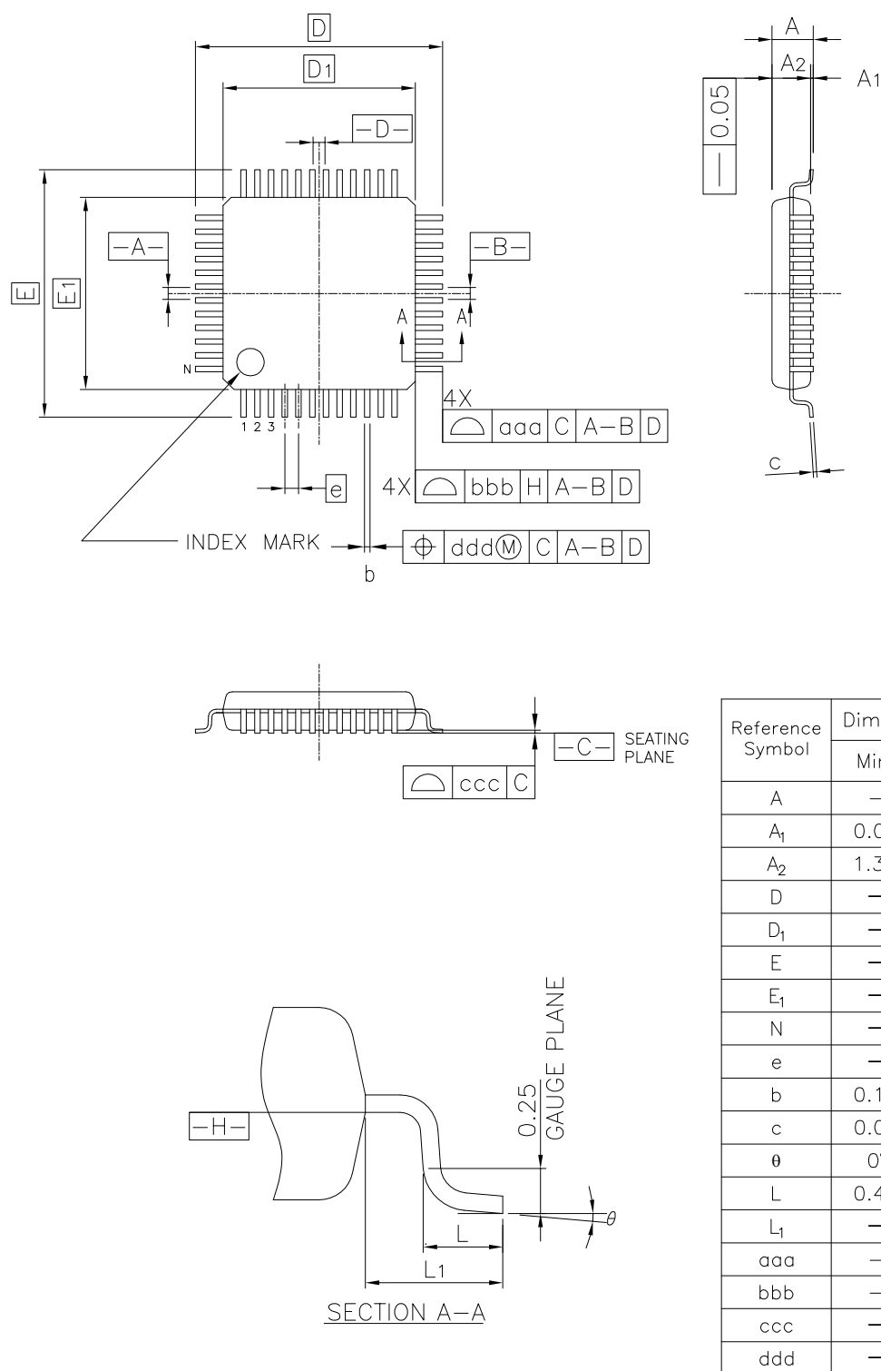
Figure 2.5 LQFP 48-pin (2)
