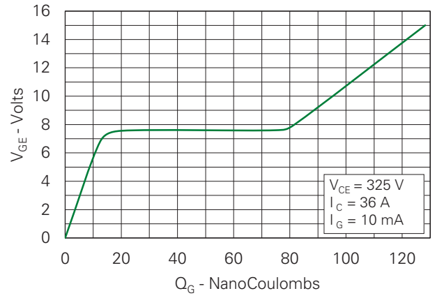
Fig. 8. Gate Charge
