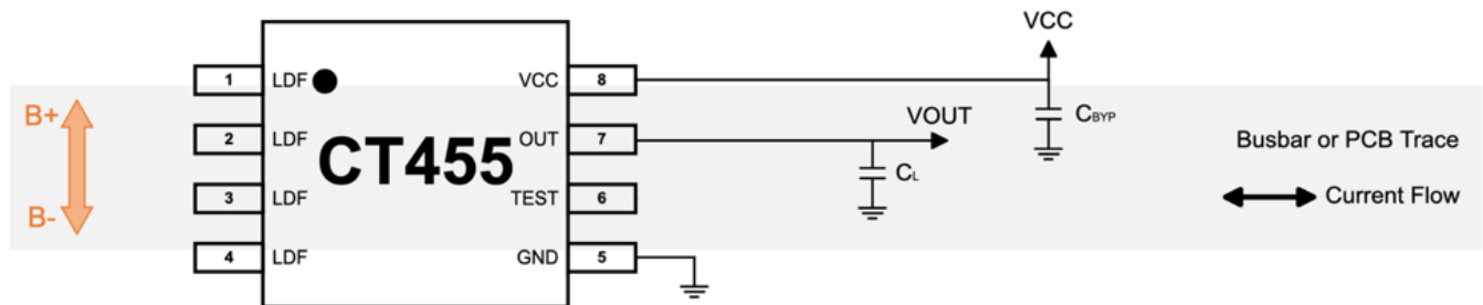
Figure 4: CT455 Application Diagram for SOIC-8
