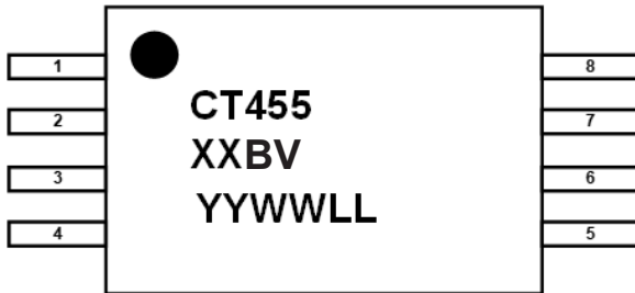
Figure 28: CT455 Device Marking for 8-Lead TSSOP Package
