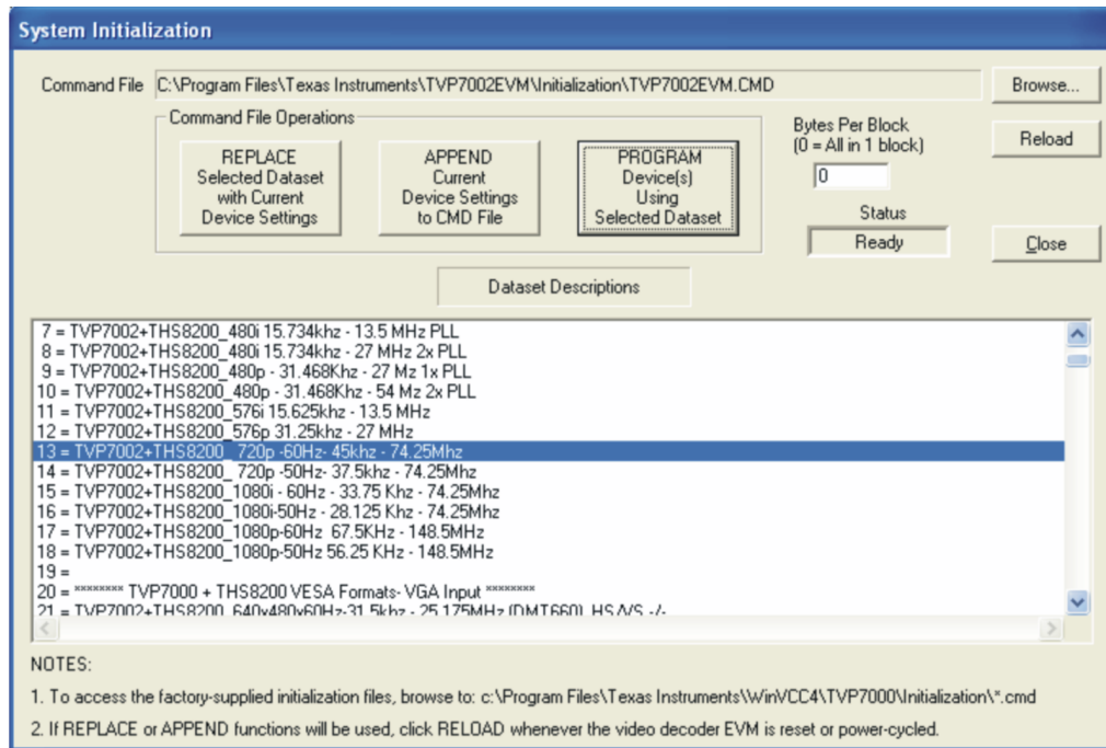
Figure 4-5. System Initialization
