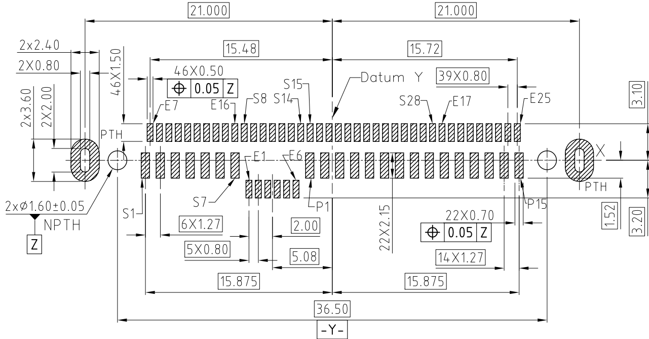
RECOMMENDED PCB LAYOUT(TOP VIEW)
