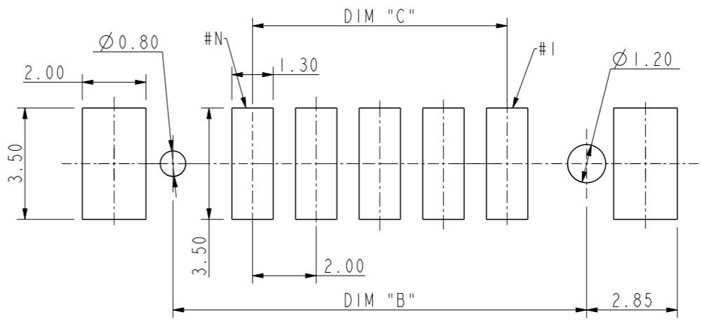
PCB LAYOUT PROPOSAL FOR RECEPTACLE 2/3/4 TOLERANCE RECOMMENDED ±0.05
