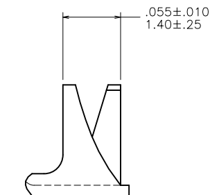
FIGURE W 32-36 AWG TERMINAL
