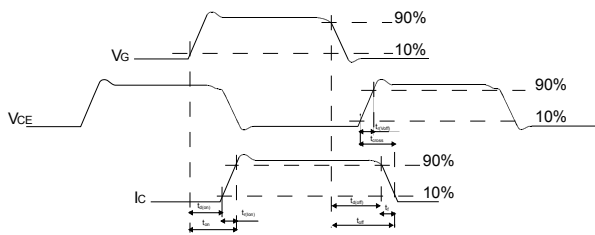
Figure 29. Switching waveform
