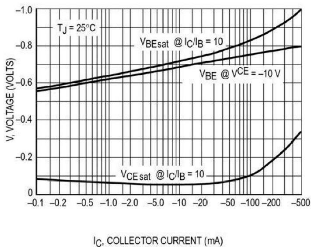
“On” Voltage
