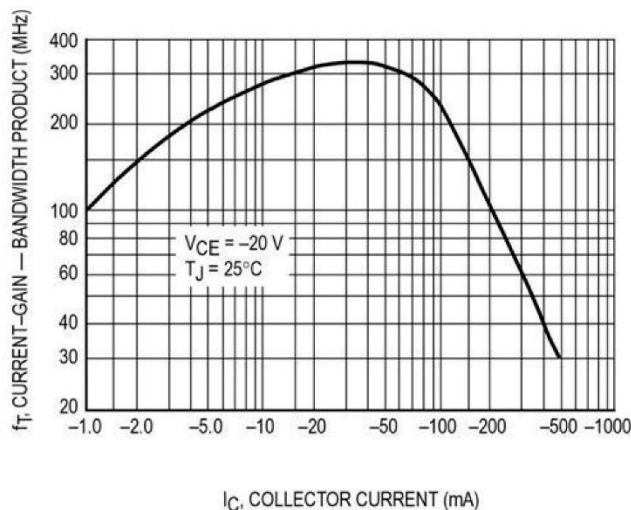
Current-Gain—Bandwidth Product
