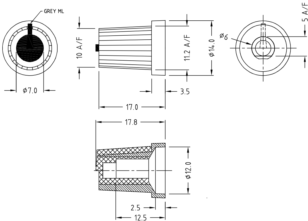
CL170805B - K85M Knob Black / Grey marker line 6mm D shaft
