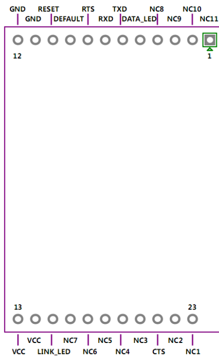
Figure 2-2 W7500S2E-R1 pinout
