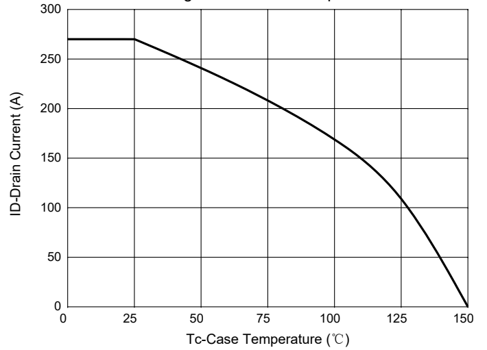
Fig. 10 - Current dissipation
