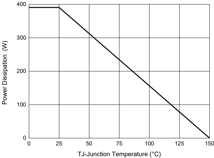
Fig.11-PD-TJ
