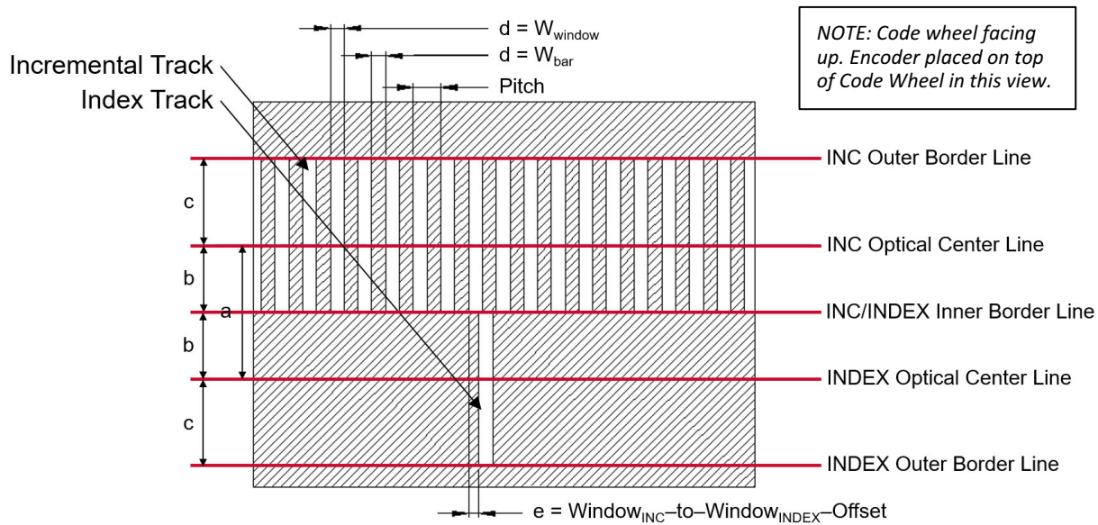
Figure 9: Code Strip Design
