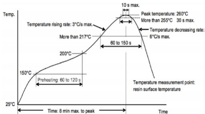
Figure 15: Recommended Lead Free Solder Reflow Soldering Temperature Profile
