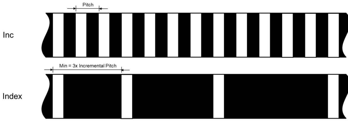
Figure 10: Multiple Index Pulse Design
