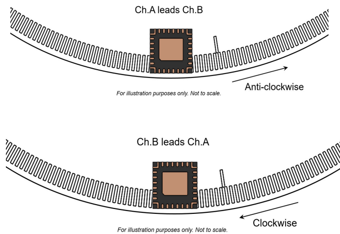
Figure 14: Channel Leads
