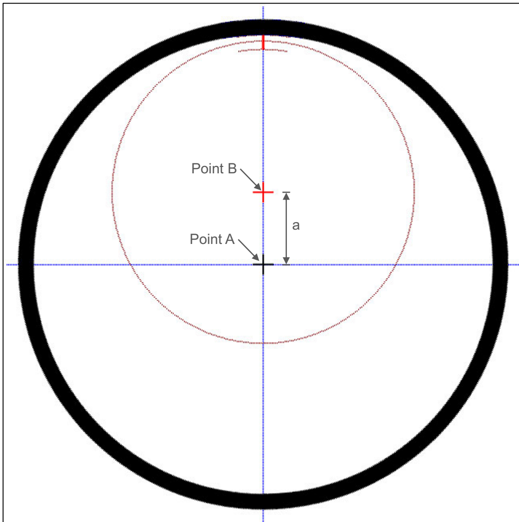
Figure 7: Code Wheel Design (A)
