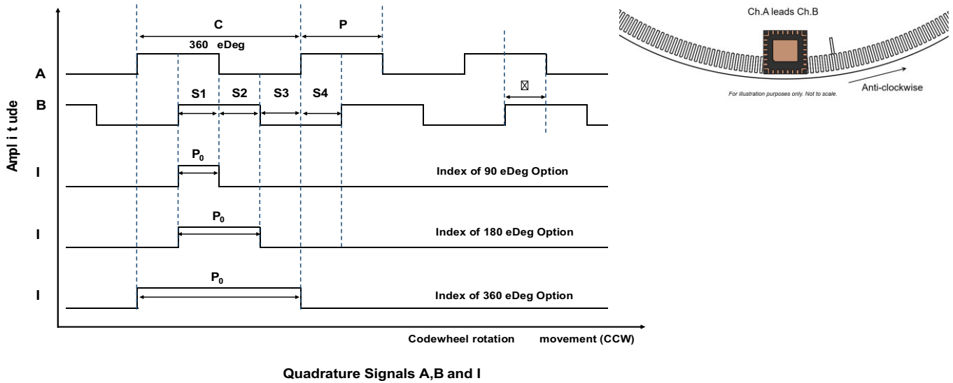
Figure 3: Digital Output Option
