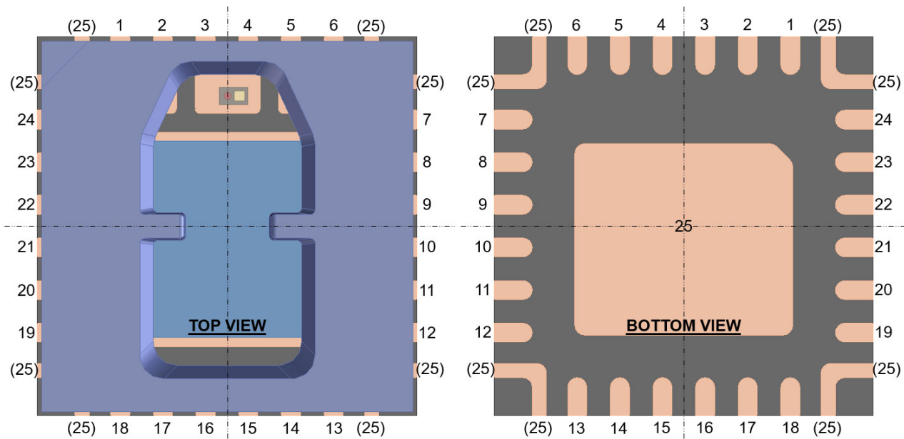
Figure 4: Encoder Pinout
