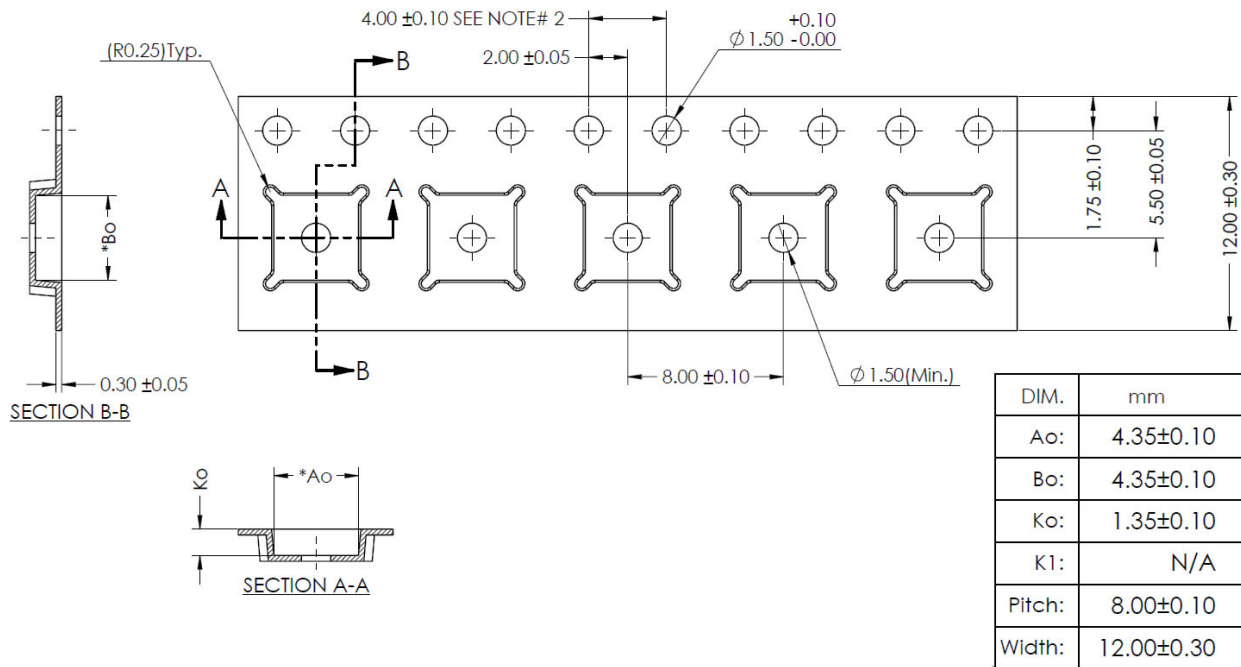
Figure 16: Tape and Reel Information
