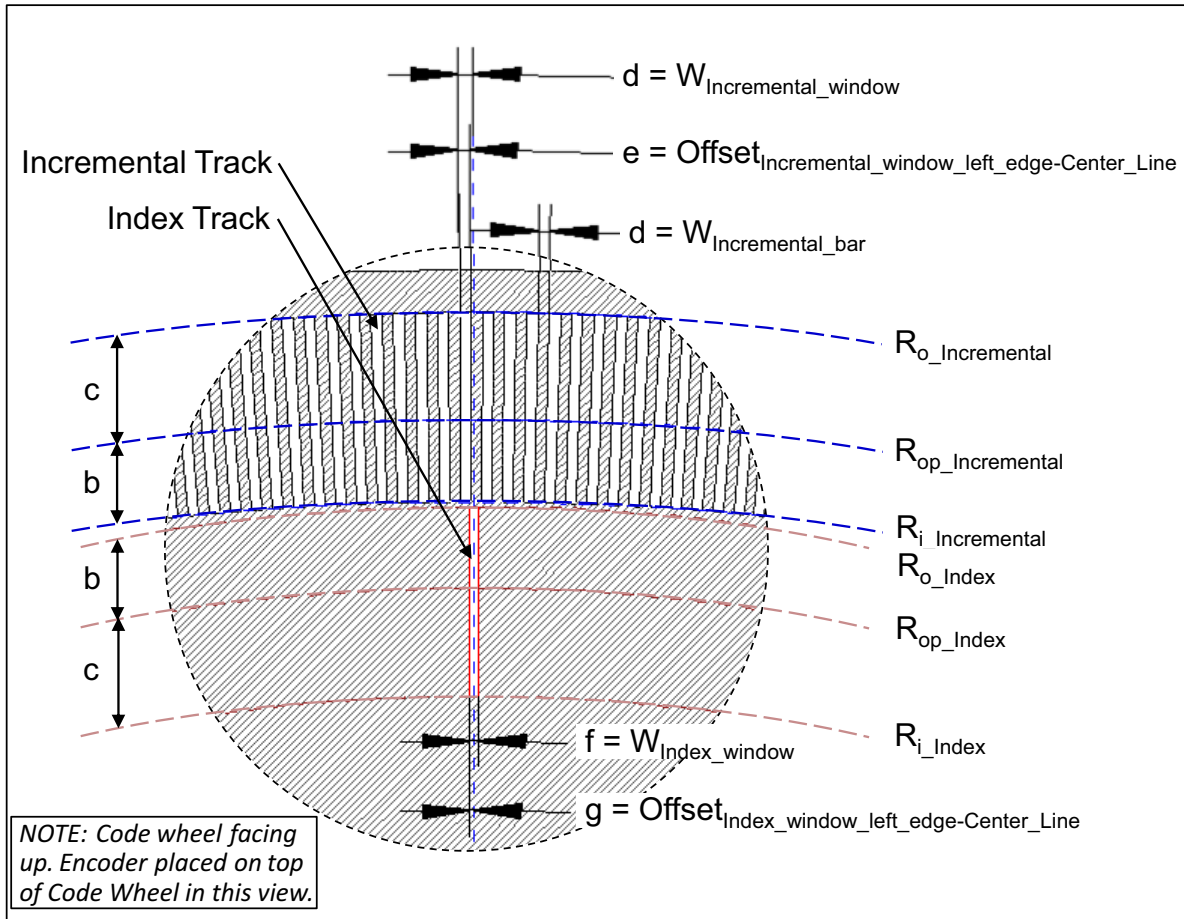
Figure 8: Code Wheel Design (B)
