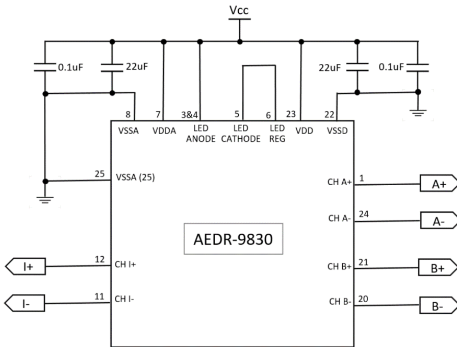
Figure 6: Connection Diagram
