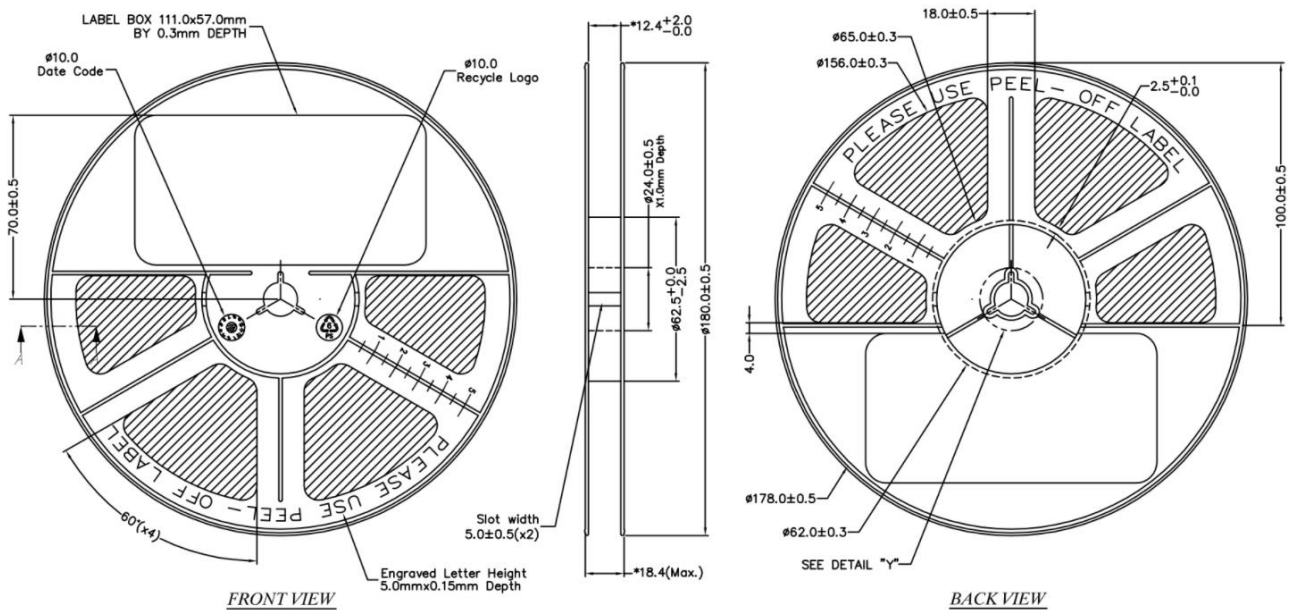
Figure 17: Reel Dimensions
