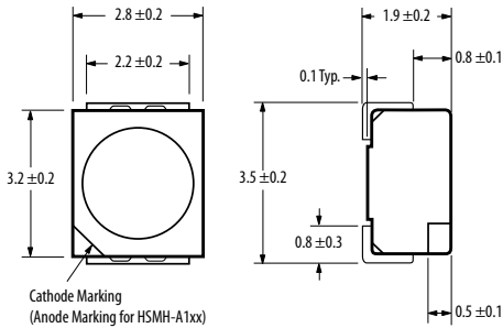
PLCC-2 Top Mount
