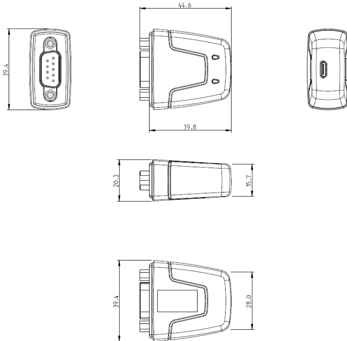
Figure 7.1 – DuoEtte Dimensions
