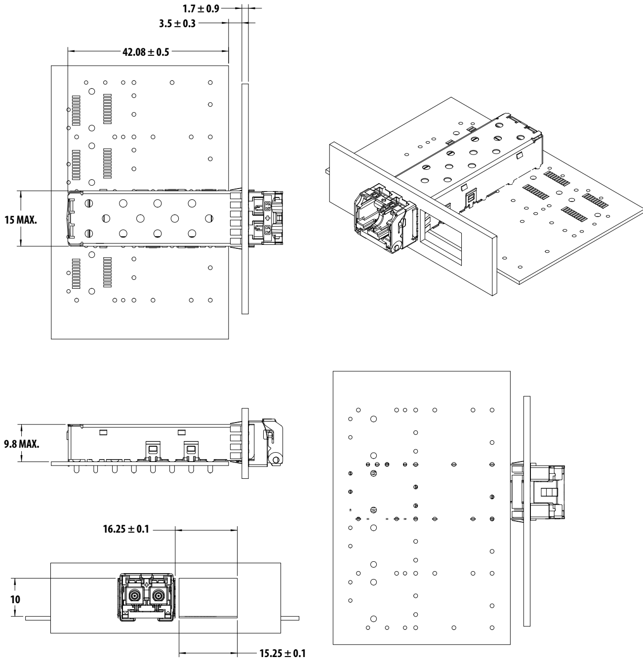
Figure 10: SFP Assembly Drawing
