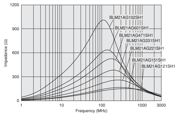
BLM21AG_SH Series
