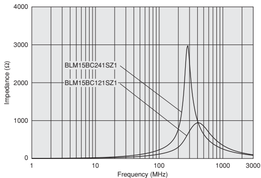
BLM15BC_SZ Series
