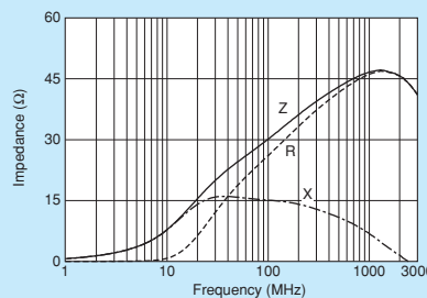
BLM15AX300SZ1
