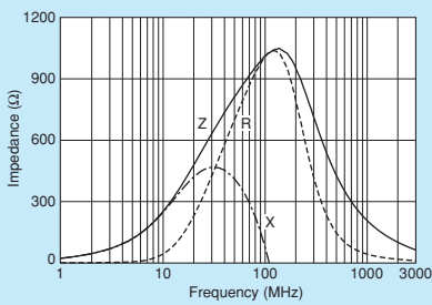
BLM15AG102SZ1/BLM15AG102SH1
