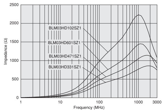
BLM03HD Series
