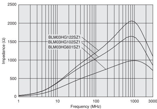
BLM03HG Series
