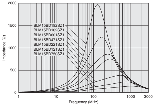
BLM15BD_SZ Series
