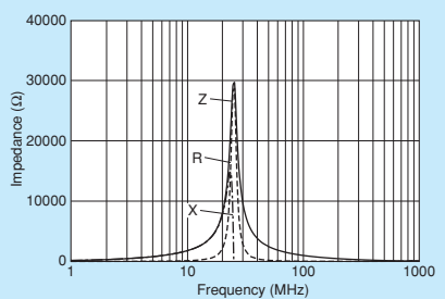
NFZ32BW151HZ11
