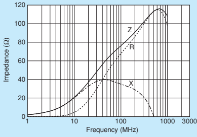
BLM15AG700SH1
