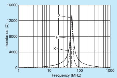
NFZ32BW520HZ11
