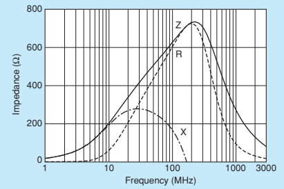
BLM15AG601SZ1/BLM15AG601SH1
