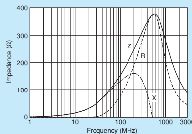
BLM18BD151SZ1/BLM18BD151SH1
