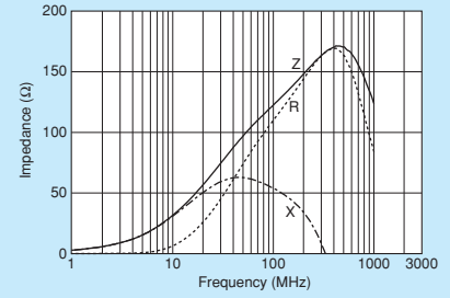
BLM15AG121SH1
