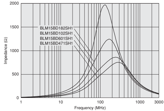
BLM15BD_SH Series
