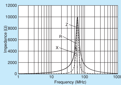
NFZ32BW310HZ11
