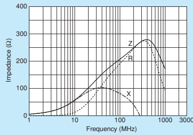
BLM15AG221SH1
