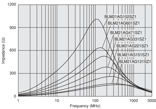
BLM21AG_SZ Series
