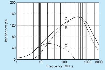
BLM18SG121TZ1
