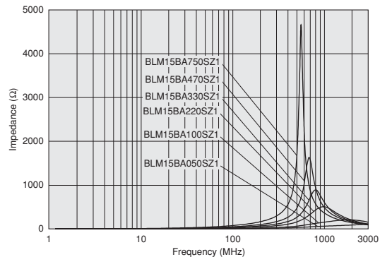
BLM15BA_SZ Series
