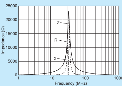
NFZ32BW101HZ11
