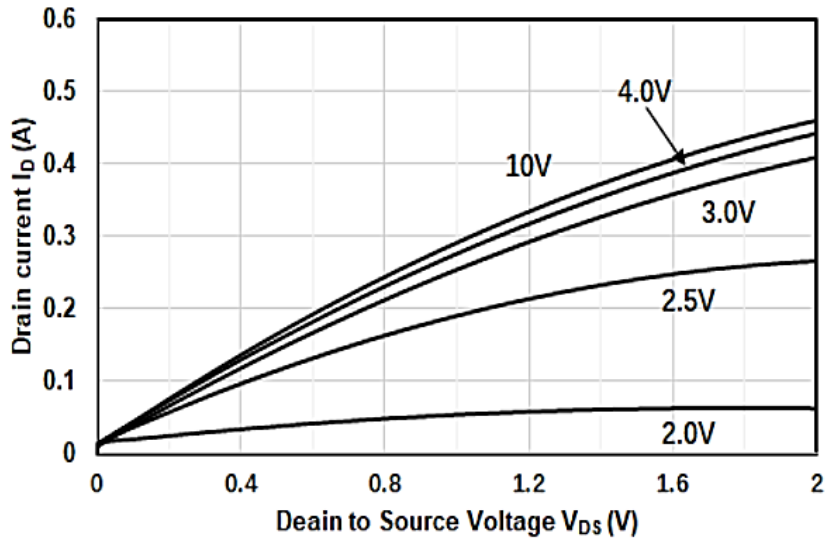
Figure 1. Output Characteristics
