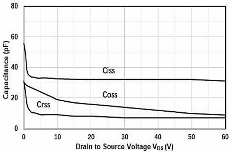
Figure 3. Capacitance Characteristics
