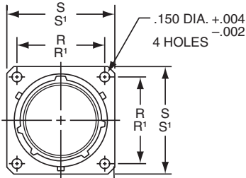
DUMMY RECEPTACLE FOR PT, SP, MS/PT CONNECTORS MS3115-XXX 10-150921-XXX
