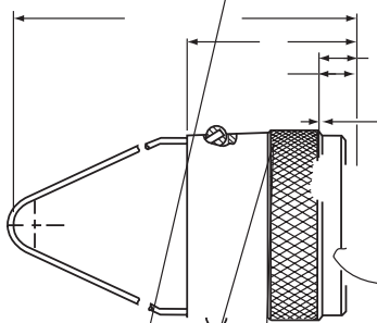
Breakaway PT-SE with Crimp Contacts, Potted Termination 71-4196XX-( ) 72-4196XX-( )
