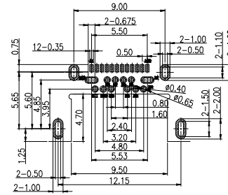
RECOMMENDED P.C.B LAYOUT(Both sides are sample) Tolerance:±0.05,Thickness=0.60mm
