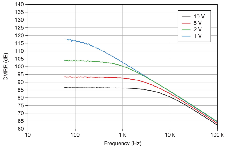
Figure 2. Common Mode Rejection Ratio versus Frequency
