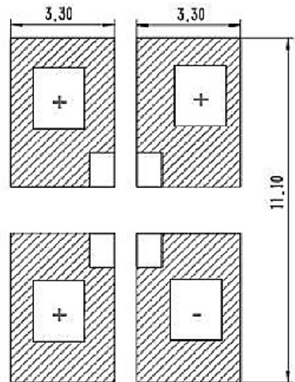
Recommended Stencil opening
