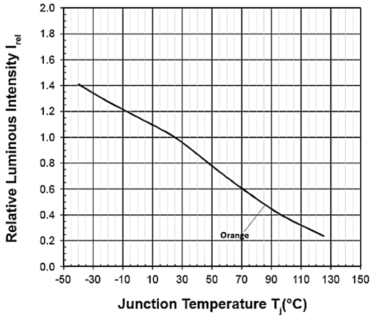
Figure 5. Junction Temperature Vs. Relative Luminous Intensity
