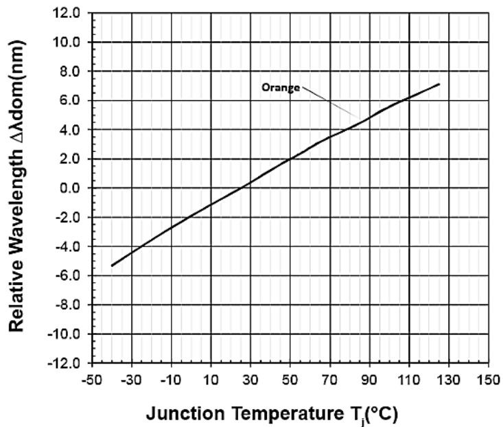
Figure 6. Junction Temperature Vs Relative Wavelength, \Delta\lambda_{dom} = \lambda_{dom} - \lambda_{dom}(25^\circ\text{C}) = f(T_j) ; IF =50mA
