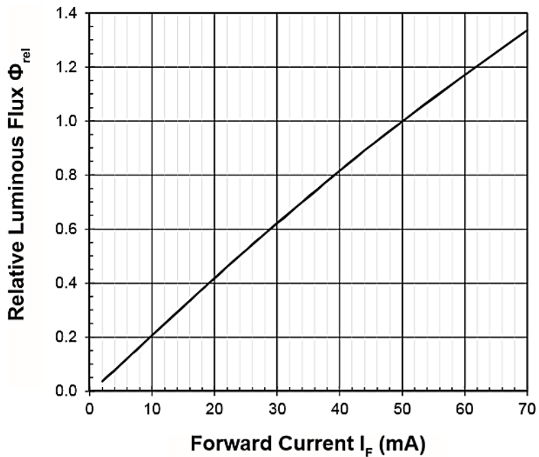
Figure 2. Forward Current Vs. Relative Intensity, \Phi_V/\Phi_V(50mA)= f(I_F)
