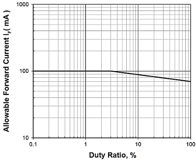
Figure 9 Allowable Forward Current Vs Duty Ratio, ( Ts = 55°C; tp ≤ 100μs)
