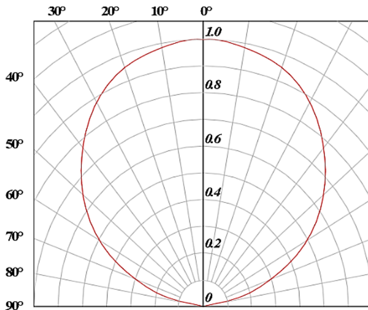
Figure 8. Radiation Diagram, I_{rel} = f(\Phi)
