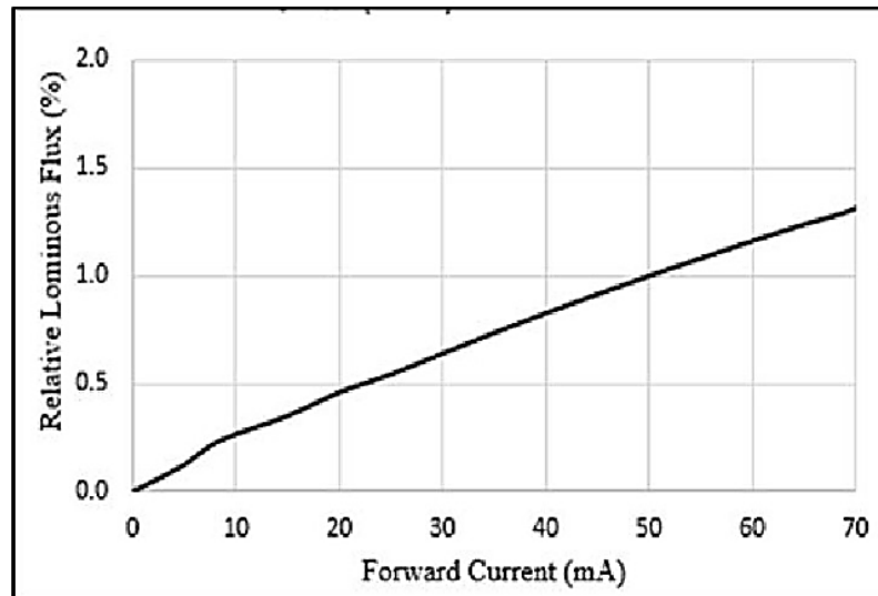
Figure 2. Forward Current Vs. Relative Intensity, \Phi_V/\Phi_V(30mA)=f(I_F)
