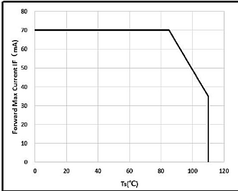
Figure 7 Ts Vs. Max. Permissible IF, I_F = f(T_s)
