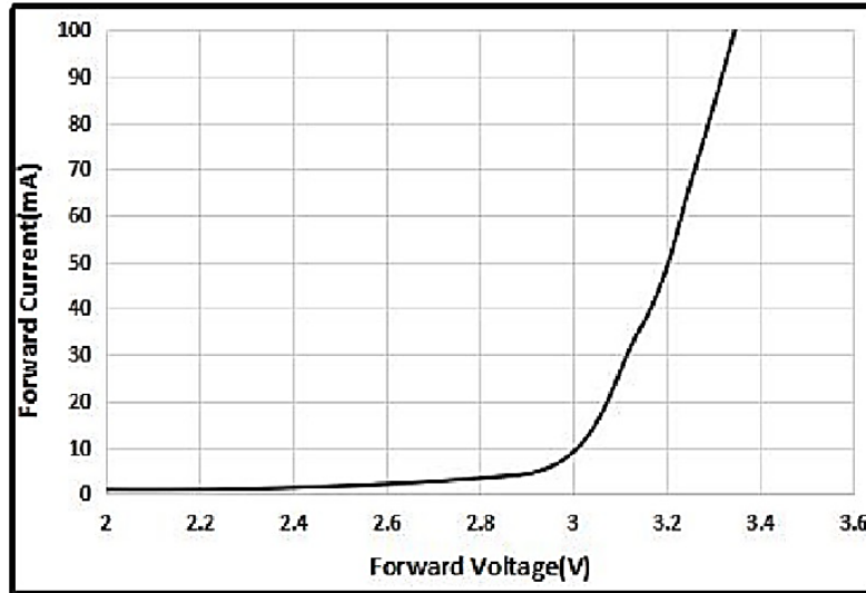
Figure 3. Forward Voltage Vs. Forward Current, IF = f (VF)
