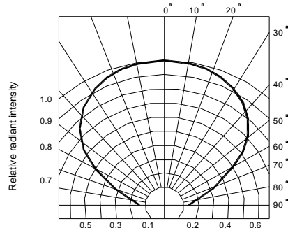
Fig.6 Radiation diagram
