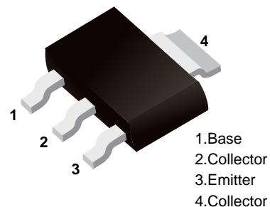
■ Simplified outline(SOT-223)
