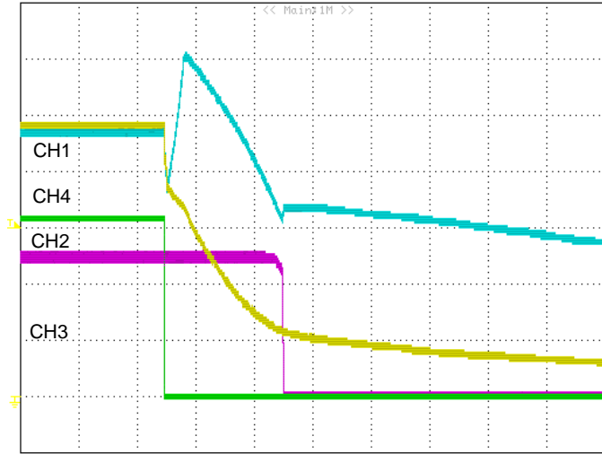
Figure 5: Hold up performance (5mS/div): CH1: Vin (VRTN_AF reference to -48V_AF, 10V/div). CH2: Iin (2A/div). CH3: 12V Vout (5V/div). CH4: VRTN_OUT reference to -48V_OUT (10V/div).
