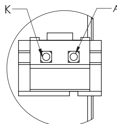
DETAIL C SCALE 8 : 1
