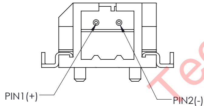
DETAILED COMPONENT A PART NO: DF3-2P-2H
