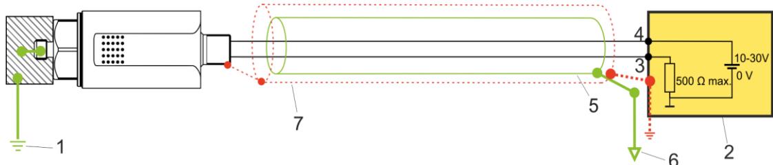
Fig. 10: Standard earthing concept
