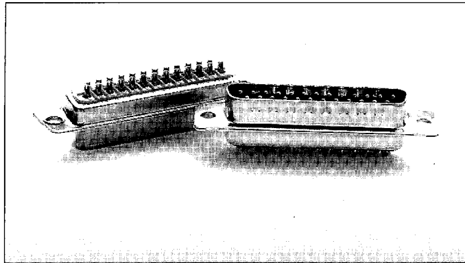
Solder cup
