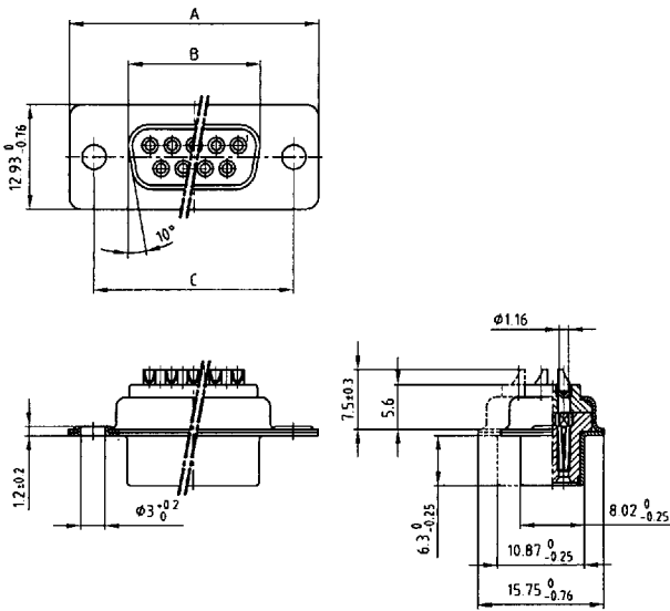
Socket connector
