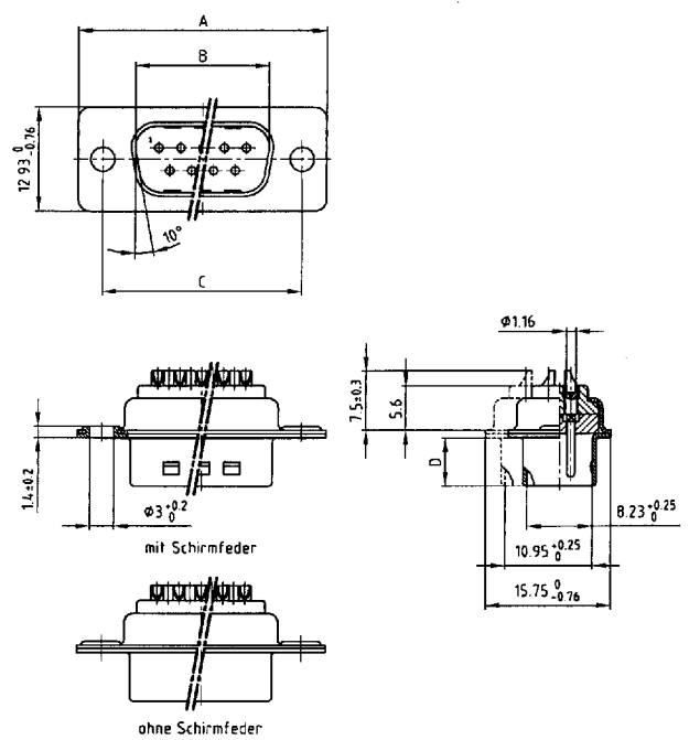
Plug connector
