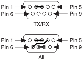
Figure 7. RS-232 Loopback
