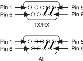
Figure 9. RS-485/422 Loopback
