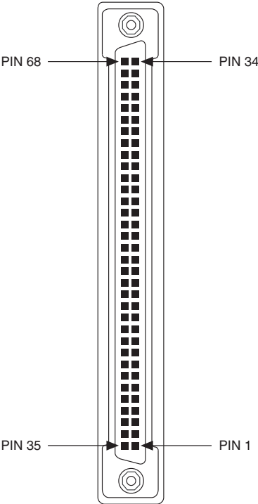
Figure 5. 68-Pin SCSI Connector Pin Locations
