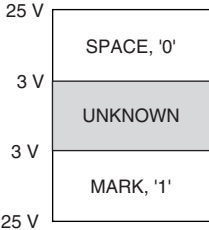
Figure 8. RS-232 Signals
