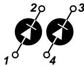
Parallel APT2X61S20J
