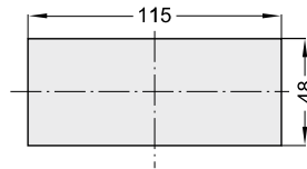
Mounting cutout
