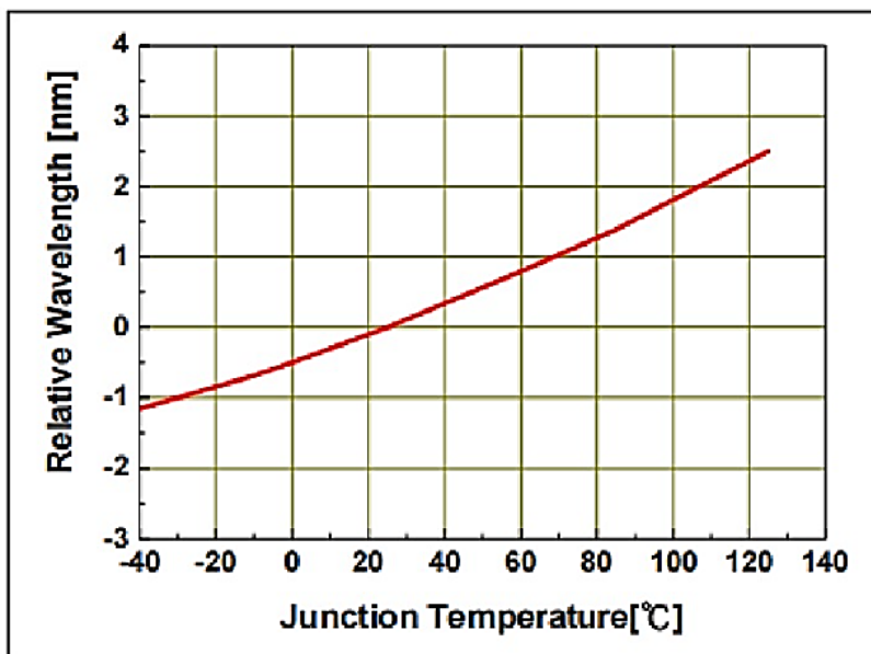
Figure 6. Junction Temperature Vs. \Delta \lambda_{dom} , \Delta \lambda_{dom} = \lambda_{dom} - \lambda_{dom} (25^\circ C) = f(T_j)
