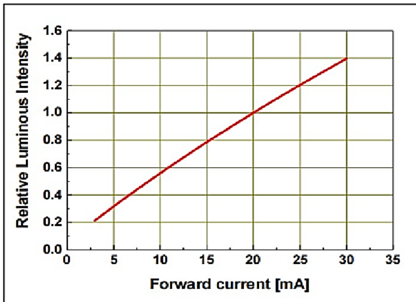
Figure 2. Forward Current Vs. Relative Intensity, \Phi_V/\Phi_V(20mA)= f (I_F)
