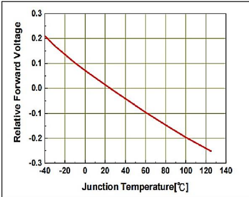
Figure 5. Junction Temperature Vs. \Delta V_F , \Delta V_F = V_F - V_F(25^\circ C) = f(T_j)
