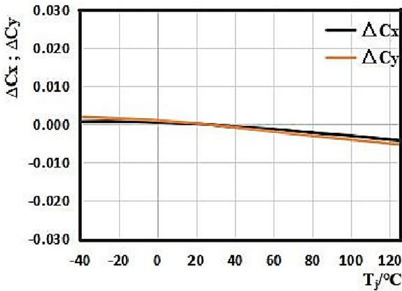
Figure 7. Junction Temperature Vs. Chromaticity Coordinate, \Delta Cx, \Delta Cy = f(Tj)
