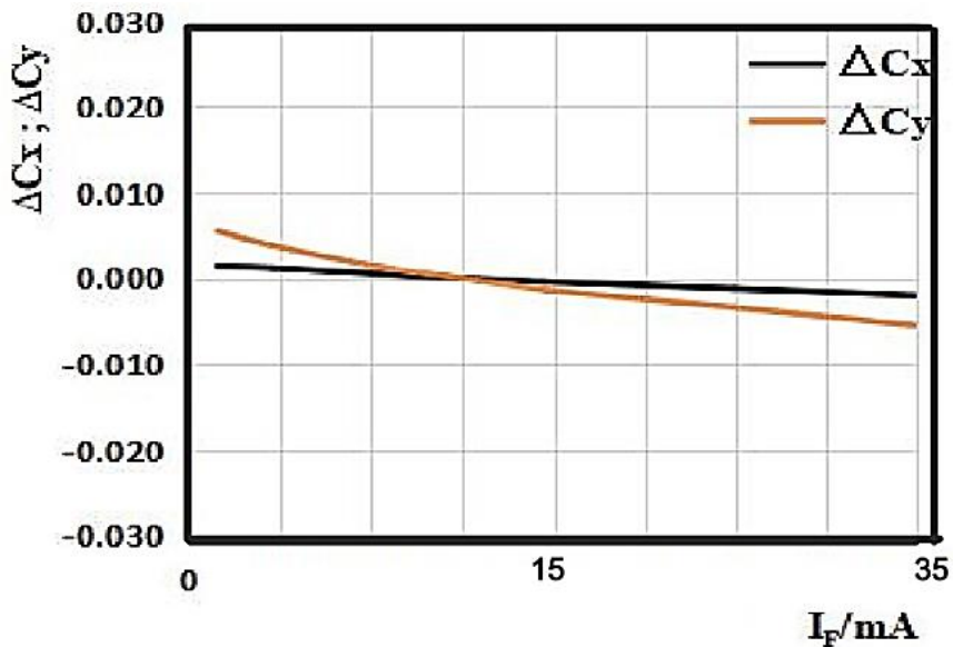
Figure 4. I_F Vs. Chromaticity Coordinate, ( \Delta C_x, \Delta C_y = f(I_F) )
