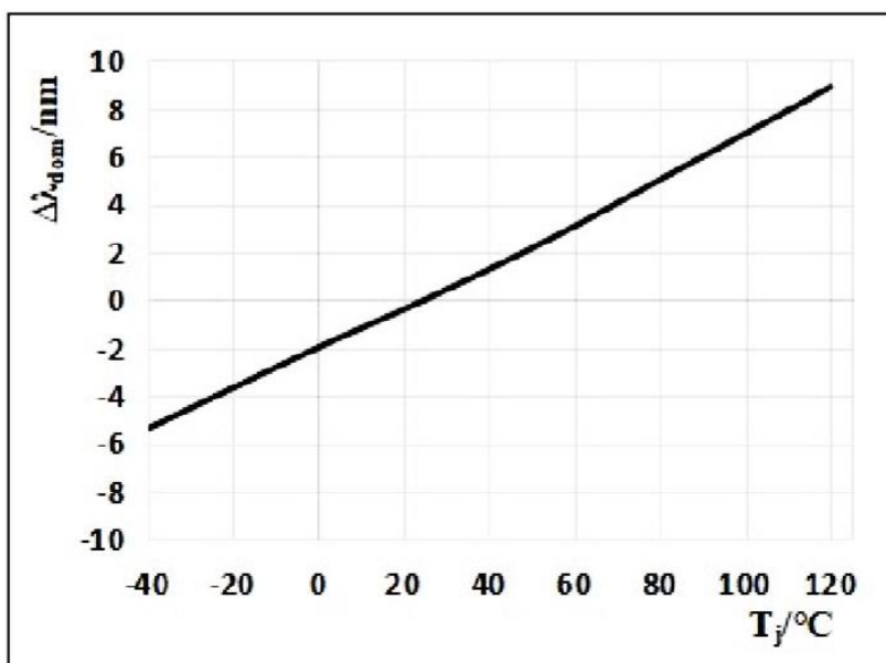
Figure 6. Junction Temperature Vs. \Delta \lambda_{dom} , \Delta \lambda_{dom} = \lambda_{dom} - \lambda_{dom}(25^\circ\text{C}) = f(T_j)
