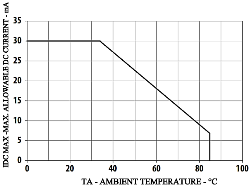
Figure 5. Maximum Forward Current vs. Ambient Temperature
