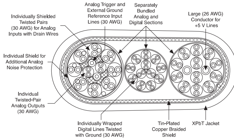
Figure 1. Enhanced-Performance Shielded Cable Used in the SHC68-68-EPM Cable
