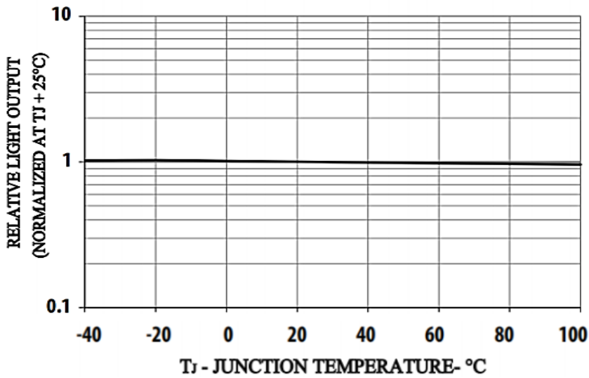
Figure 7. Relative Light Output vs. Junction Temperature
