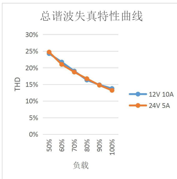
Total harmonic distortion characteristic curve
