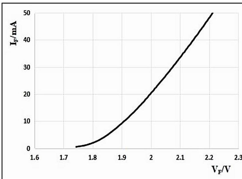
Figure 3. Forward Voltage Vs. Forward Current, I_F = f(V_F)
