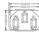
(IEC 60320, C13, 13A 250V~) (Dimensions of Connector Face)
