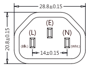
(IEC 60320, C14, 13A 250V~) (Dimensions of Plug Face)
