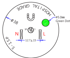
(NEMA 5-15P, Hospital Grade) (Dimensions of Plug Face)
