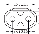
(IEC 60320, C7, 10A 125V~) (Dimensions of Connector Face)
