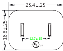
(NEMA 1-15P, NP) (Dimensions of Plug Face)
