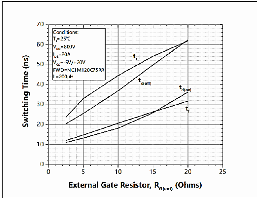
Figure 25. Switching Time vs. R_{G(\text{ext})}
