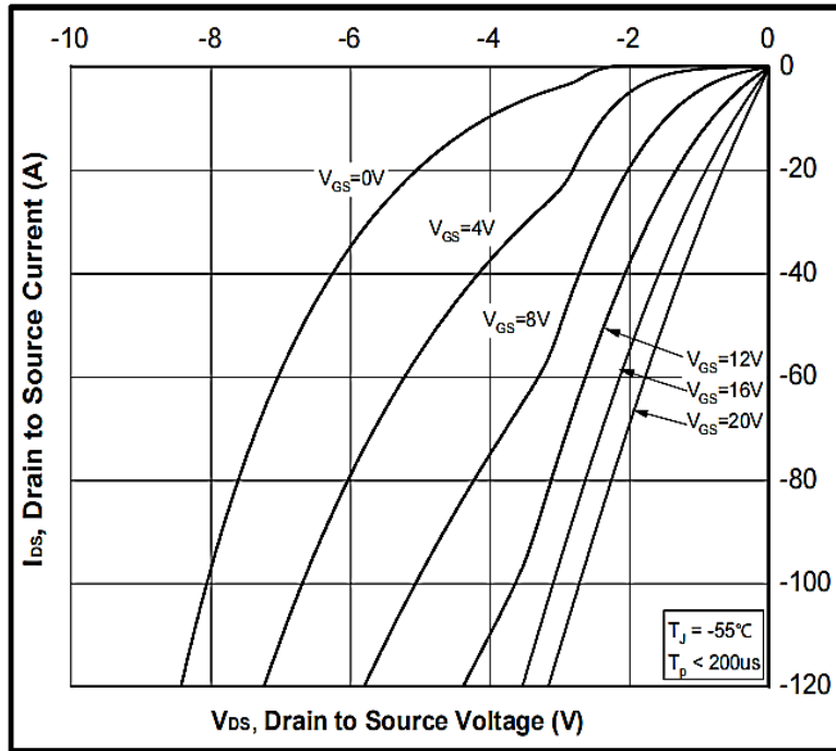
Figure 13. 3 rd Quadrant Characteristic at -55^\circ\text{C}
