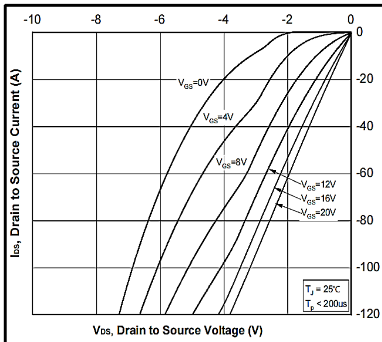
Figure 14. 3 rd Quadrant Characteristic at 25^\circ\text{C}
