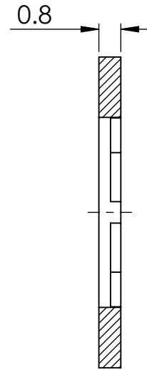
SECTION Y-Y
