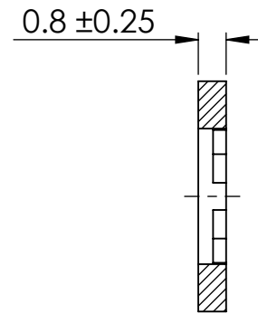
SECTION Y-Y
